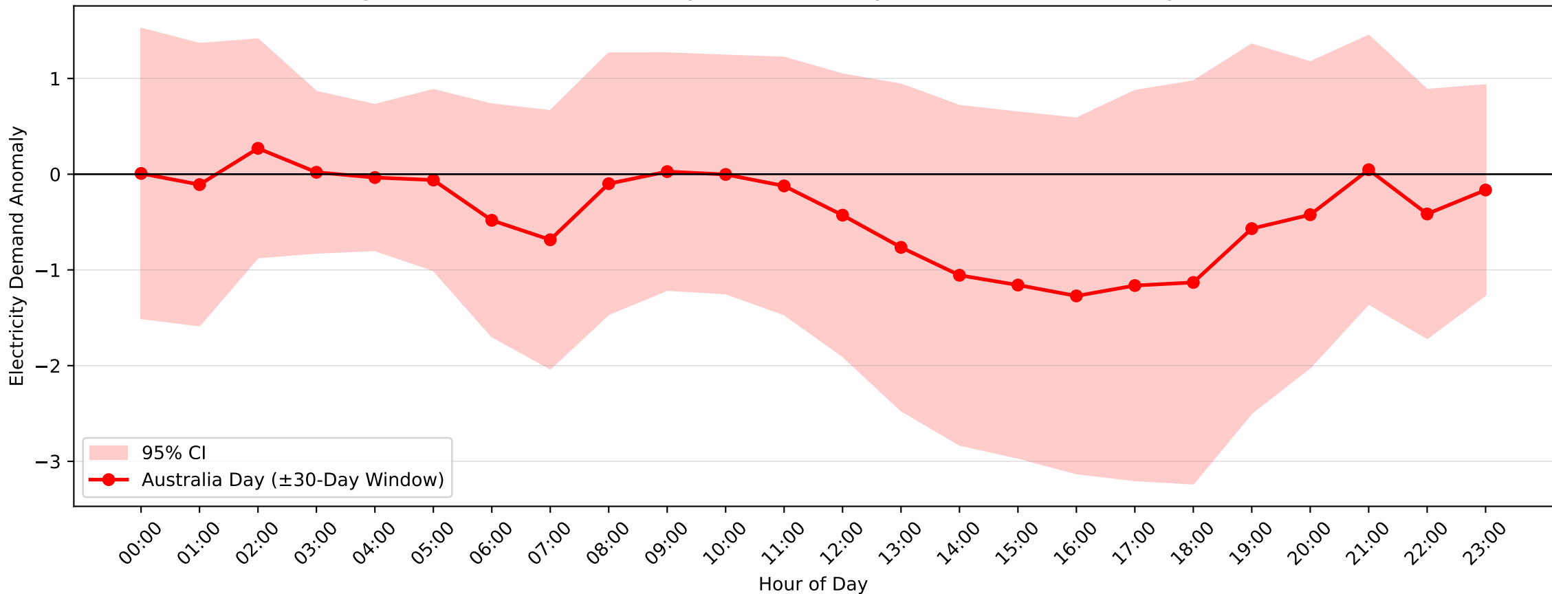
Edgeworth Demand Anomaly: Australia Day (2004-2017, \pm 30 -Day Window)
